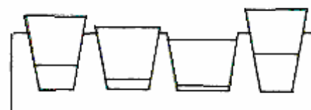
Unequal machined pulley grooves
